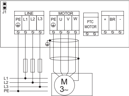
Fig.4 Size B
