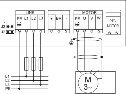
Fig.6 Size D
