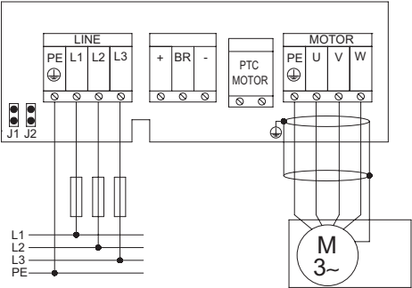
Fig.5 Size C
