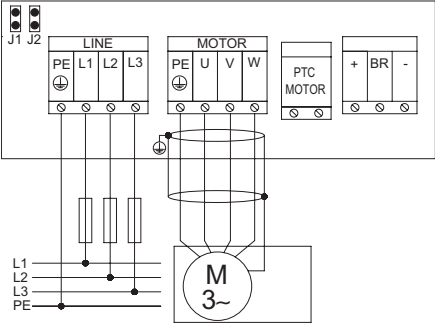
Fig.3 Size A
